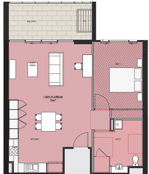
One-bedroom unit floor plan.
